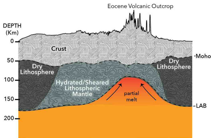
Fig. 3. A schematic cartoon of the key tectonic elements inferred from our model.
